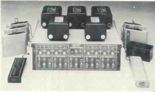
An example of the Frezzolini multicharger used by ABC charging 13 batteries simultaneously.
